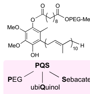
Figure 1. Components of PQS.
