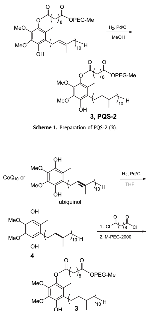
Scheme 2. Alternative route to preparation of PQS-2 ( 3 ).
