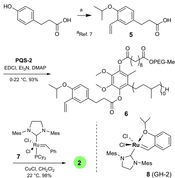
Scheme 3. Preparation of PQS-2-attached GH-2 catalyst 2 .
