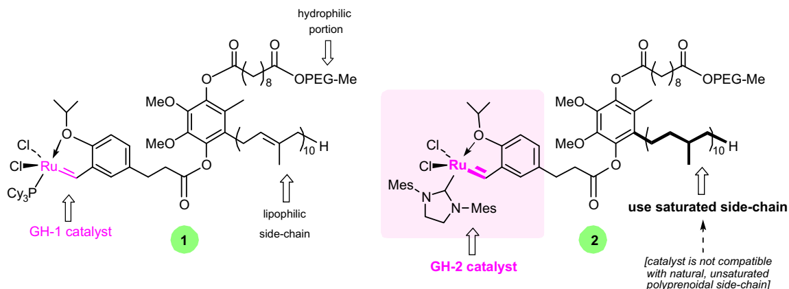
Figure 2. PQS-attached Grubbs–Hoveyda metathesis catalysts 1 and 2 .
